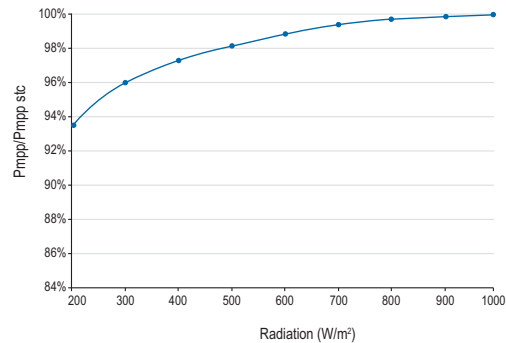
Weak light performance at Pmpp — Siiiken module's average
